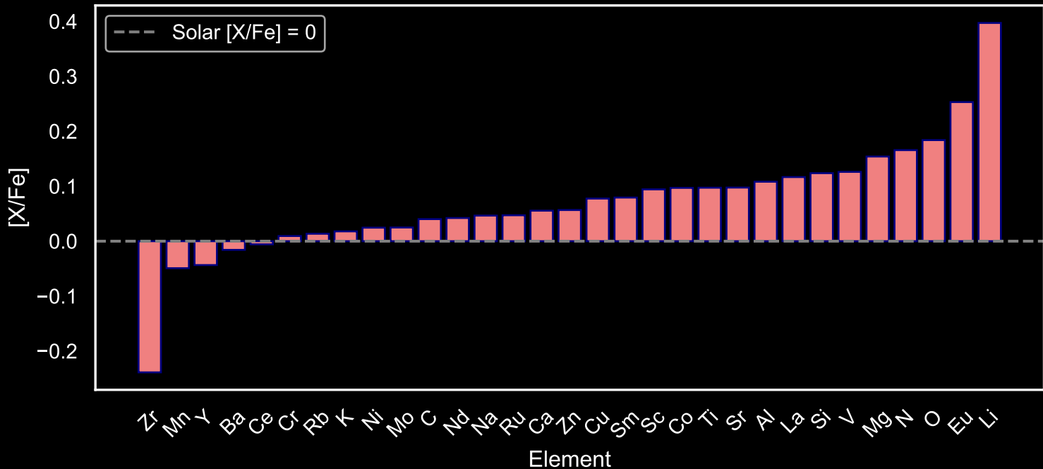
Abundance Pattern for GALAH Star Field [56] (N=301)
