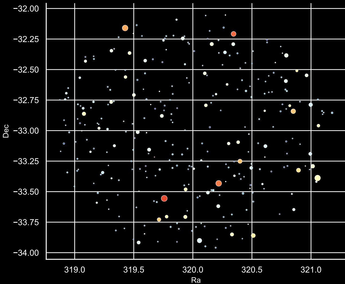
Field [56] Ra [319.96] Dec [-33.01] Stars: 301
