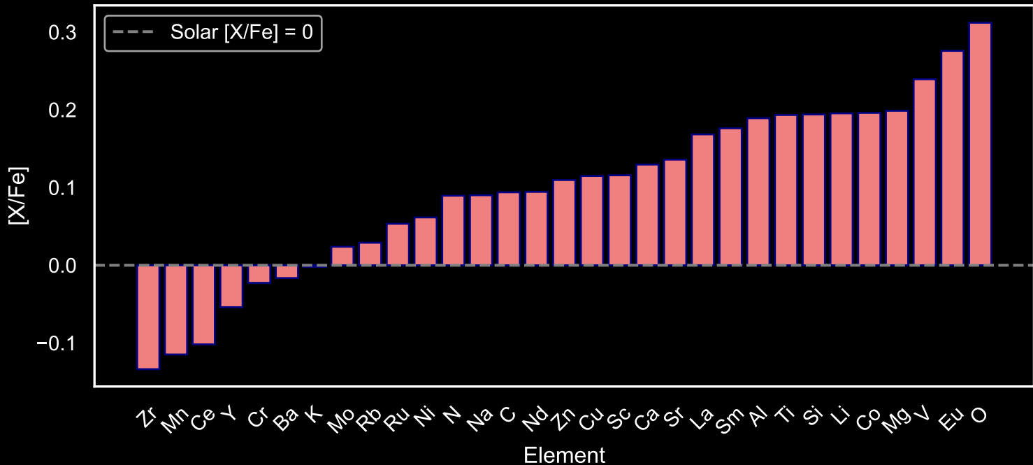
Abundance Pattern for GALAH Red Giants: Star Field [56] (N=71)
