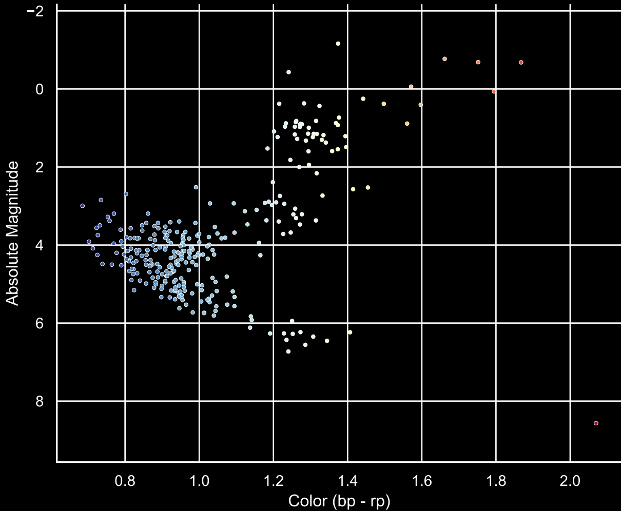
GALAH Hertzprung-Russel Diagram Field [56] Ra [319.96] Dec [-33.01]
