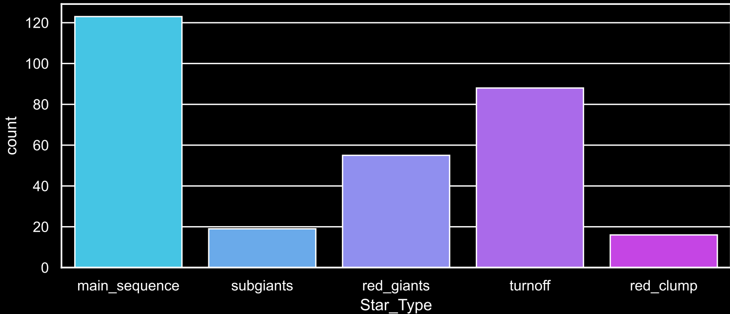
Field [56] Count plot of Star Type
