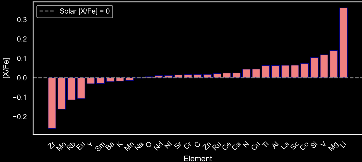
Abundance Pattern for GALAH Main Sequence Stars: Star Field [56] (N=123)
